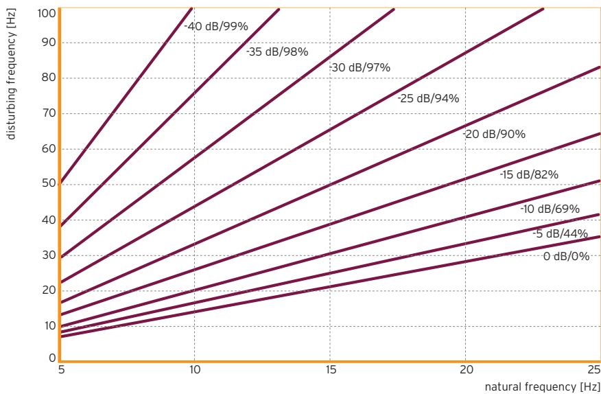
Figure 4: reduction of the transmitted mechanical vibrations by implementation of an elastic bearing consisting of Sylomer® SR 1200
