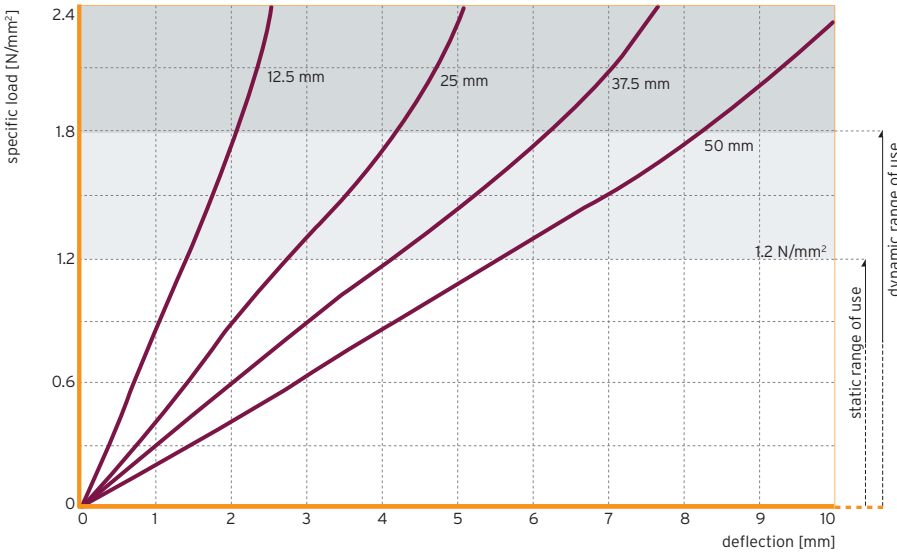
Figure 1: Quasistatic load deflection curve measured with a loading rate of 0.12 N/mm 2 /s
